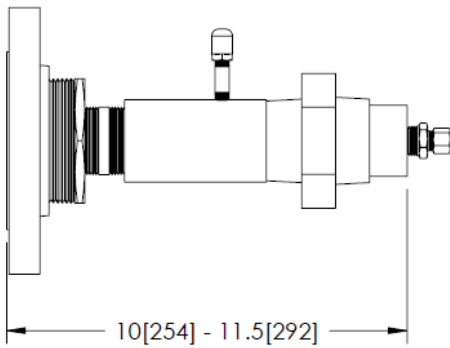
FIBEROPTIC FLANGE MOUNT
